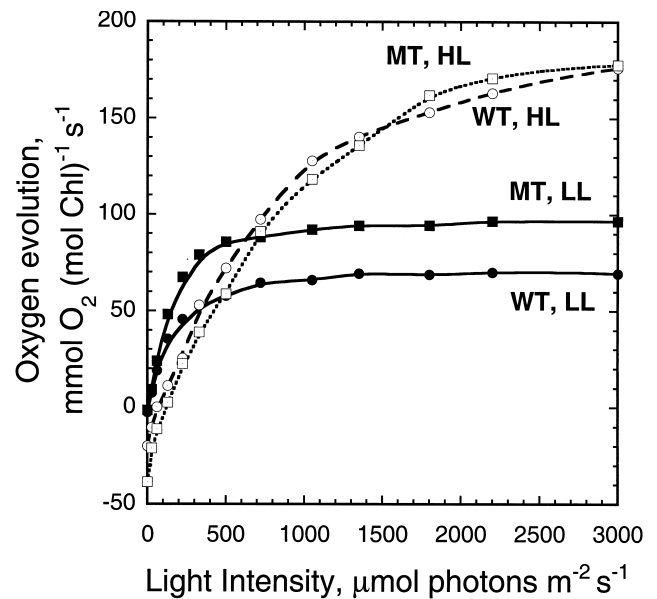
Fig. 6. The light saturation curves of photosynthesis in LL-grown wild-type (●), LL-grown mutant (■), HL-grown wild-type (○) and HL-grown mutant (□) D. salina . Rates of oxygen evolution on a per chlorophyll basis were measured as a function of actinic light intensity.
